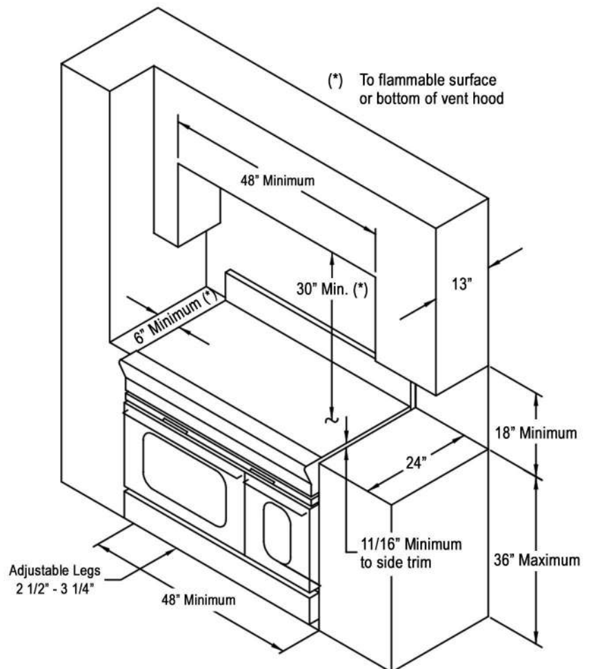
CLEARANCES
