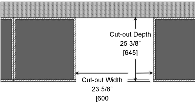
Installation Cut-out (Plan View)
