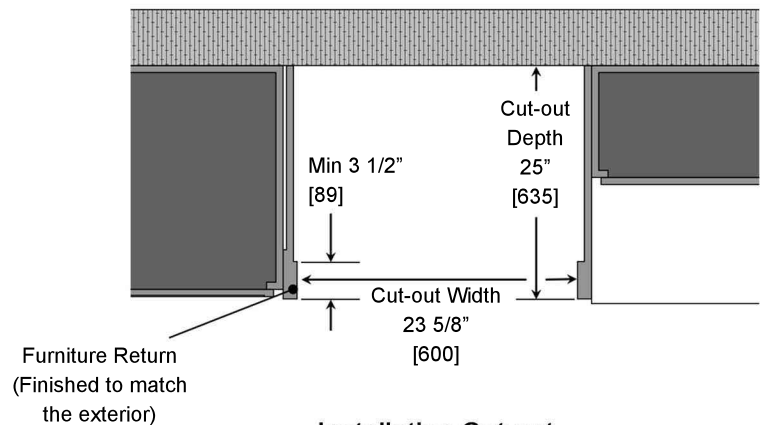
Installation Cut-out (Plan View)
